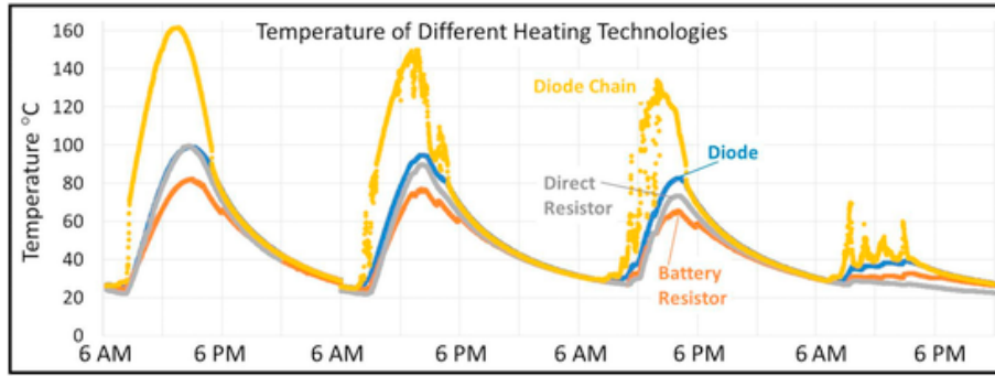
Fig. 5. Each solar panel powered a different heating technology in three insulated cook pots (Fig. 4) containing 3L of water. The graph shows the temperature of the water in each cookpot as well as the temperature of the diode chain (yellow) on the diode-heated pot. The first day of near perfect sunlight is discontinuous (cut at 6 a.m.) from the following three consecutive days of diminishing sunlight intensity.
