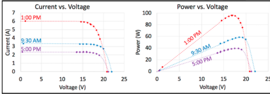
Fig. 6. Calibration of (nominally) 12V, 100W solar panels under three different solar intensities. Reduction of solar intensity reduces the current, but not the voltage. The maximum power voltage stays relatively constant under all intensities at about 17V. The dotted trend lines are provided as a guide to the eye.
