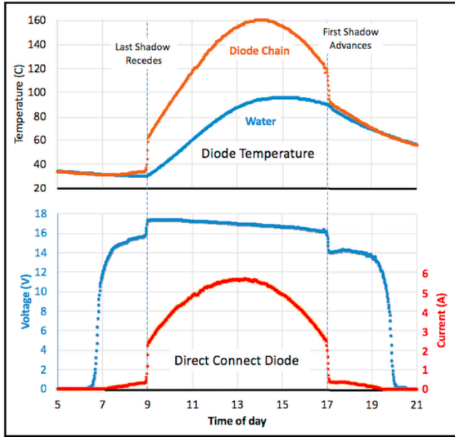
Fig. 8. Below, the voltage (blue) and current (red, axis at right) from the solar panel connected to the diode-heated cookpot. The graph above shows the evolution of cookpot water temperature as well as the temperature of the diode chain itself.
