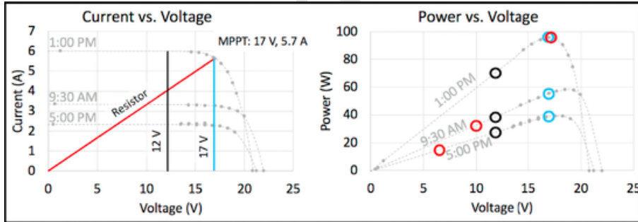
Fig. 7. Left: A resistor connected to a solar panel (red) receives increased voltage for higher solar intensities. In contrast, at all solar intensities an idealized charge controller (black) extracts power from the solar panel at 12V, and an idealized diode chain (blue) can extract power near MP, the maximum power point. Right: The diode heater and resistive heater both draw the maximum power under full sunlight, but the power drawn by the resistive heater drops off more with reduced solar intensity than that of the diode and charge controller.
