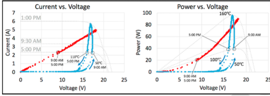
Fig. 10. The real behavior of the direct-connect resistive heater (red) and the diode heater (blue) depicted in Fig. 7.
